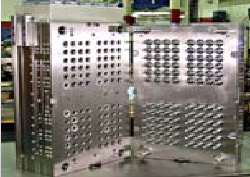
96 cavities injection mould
