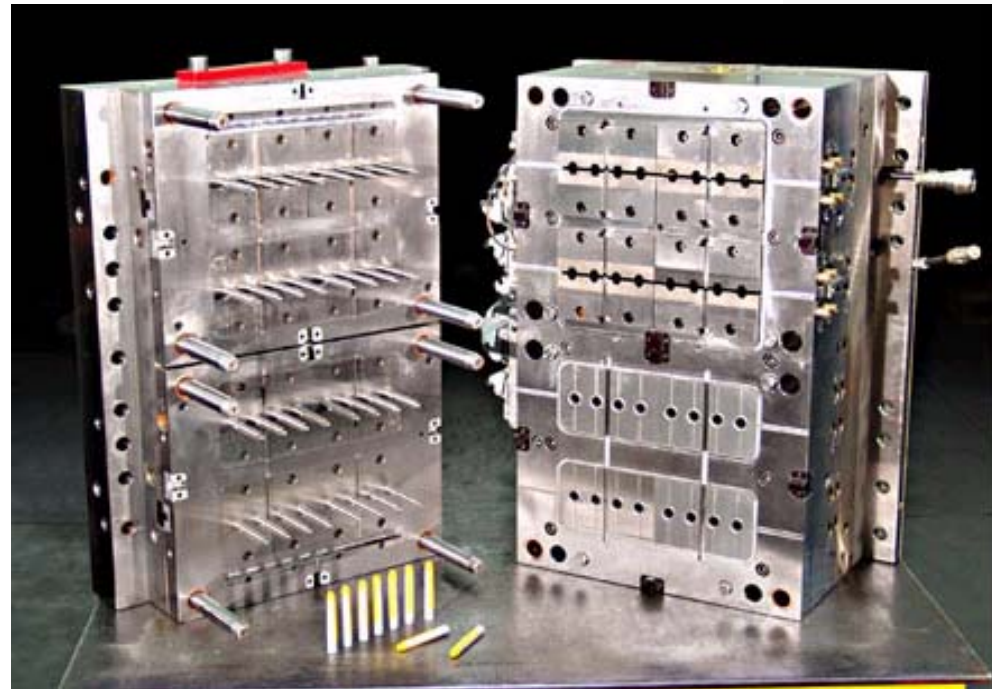
16+16 double injection mould
