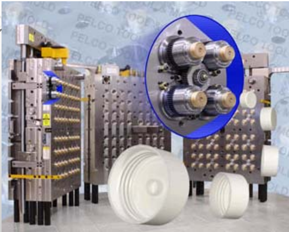
Muti-cavity stack injection mould
